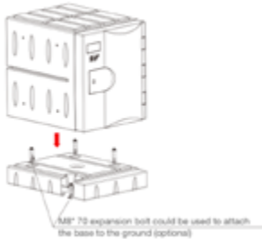
Schematic diagram with ground
